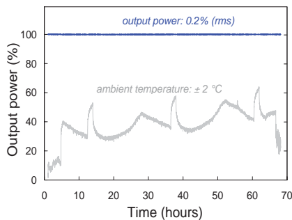
Long term stability. Output power and ambient temperature over 70 hours showing power fluctuations of 0.2% rms
