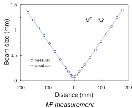
Output beam profile
